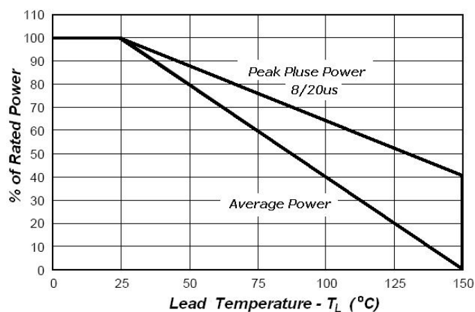
Fig2. Power Derating
